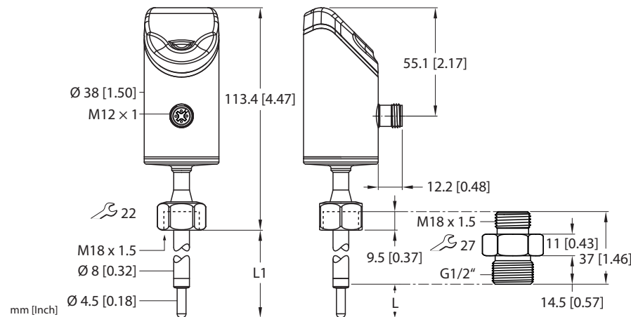
Abb. 3: Abmessungen in mm [Zoll]
