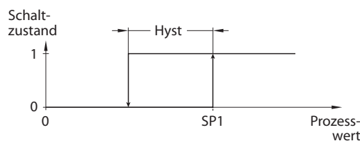
Abb. 4: Single Point Mode
