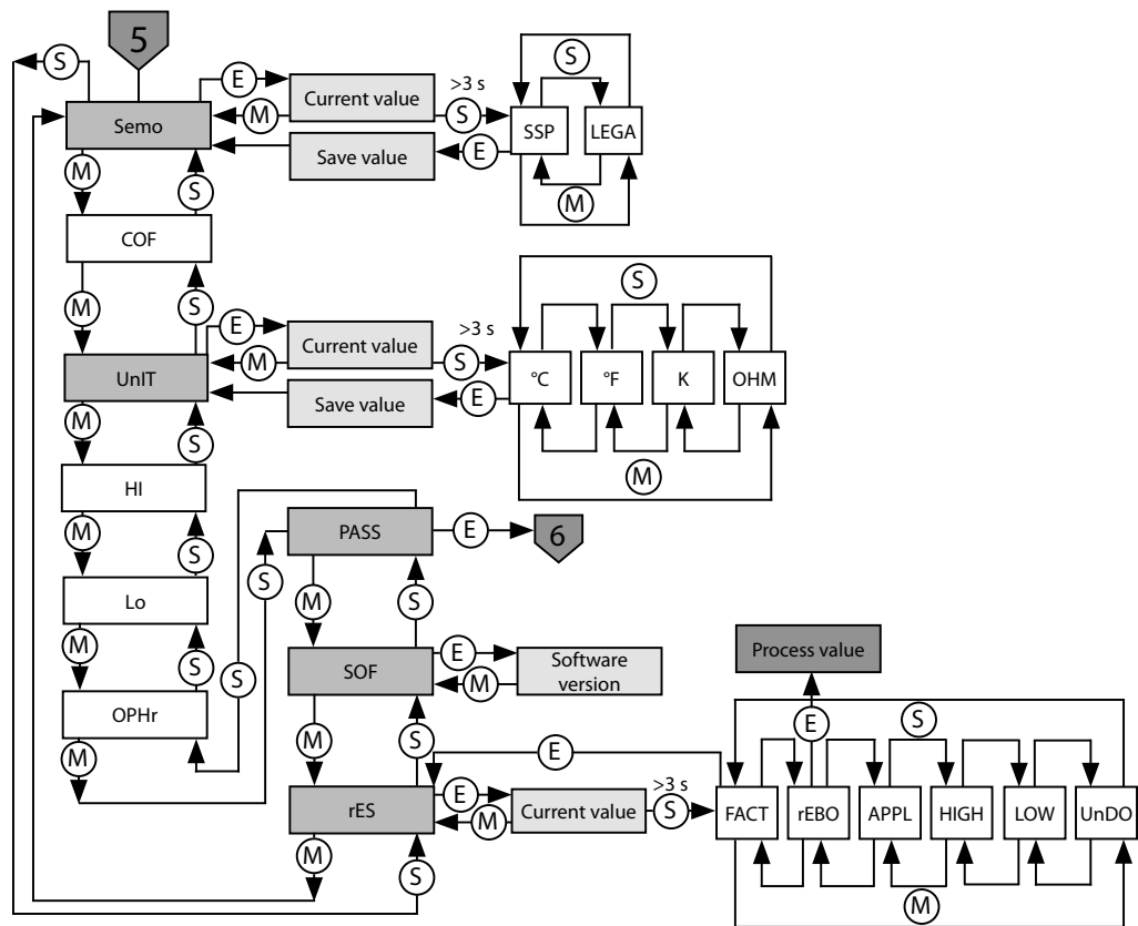
Abb. 23: Untermenü Extended-Functions (EF)
