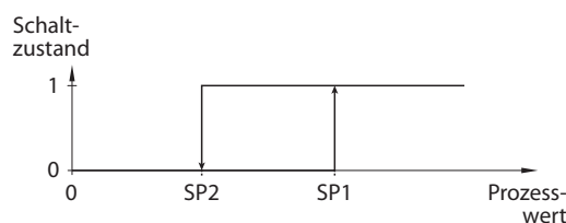
Abb. 5: Two Point Mode
